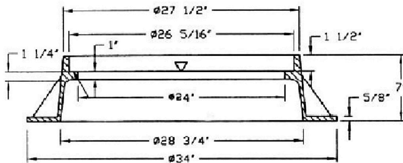
FRAME SECTION
