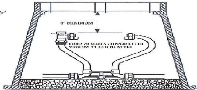
COMPANION METER BOX WITH COPPER SETTER (FOR SETTER DETAILS SEE STANDARD DRAWING 172)
