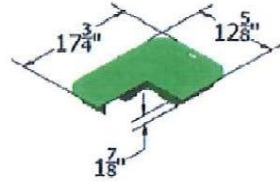
1520 T COVER HDPE BLACK
