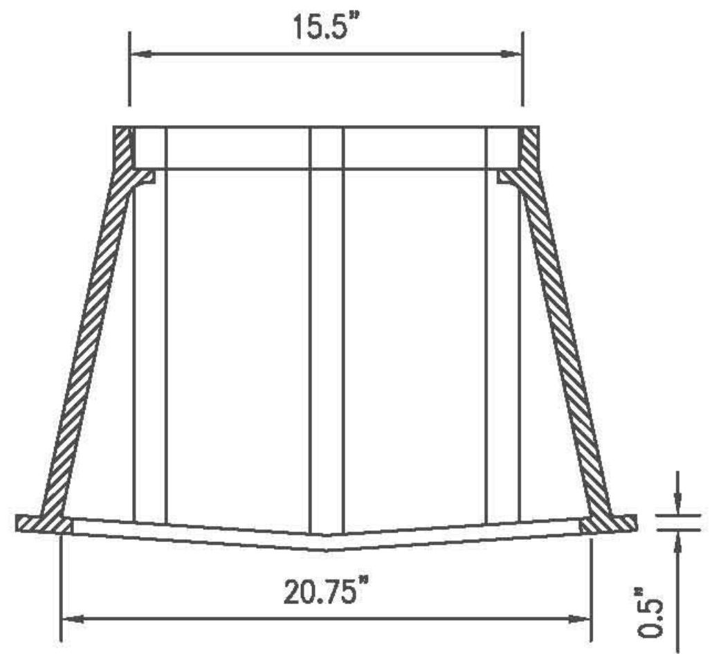
LONG SIDE VIEW
