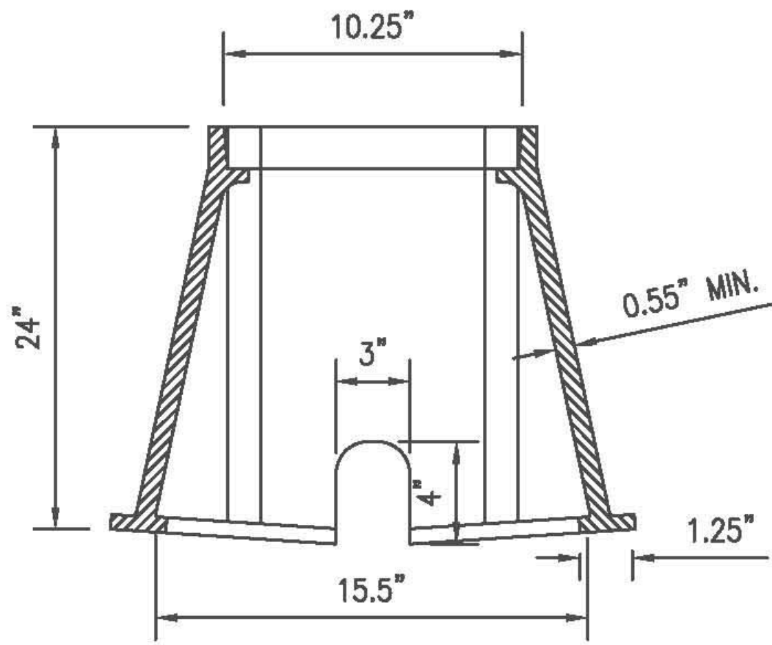
SHORT SIDE VIEW
