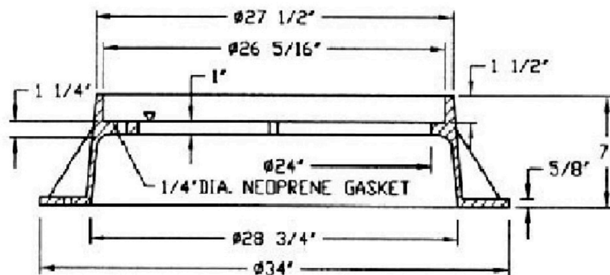
FRAME SECTION X-X
